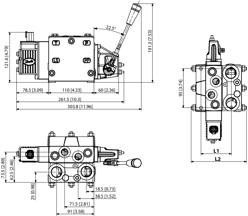
PVB 16 dimensions (12 sections)
